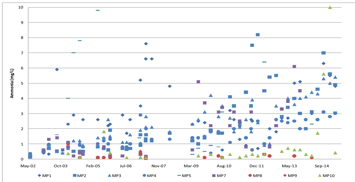
Figure 9.3 Groundwater, dredge pond water, Georges River surface water and storm water ammonia results (reduced scale)
